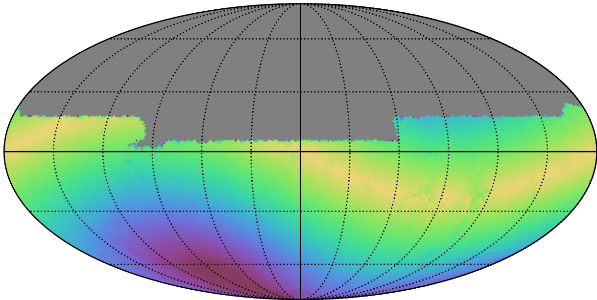
noroll_mjdp60_v3.4_10yrs All sky u band: Max solarElong
