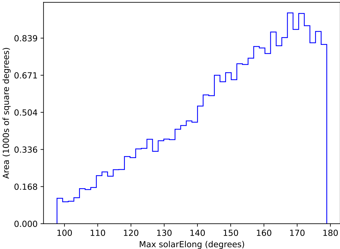
noroll_mjdp60_v3.4_10yrs All sky u band: Max solarElong
