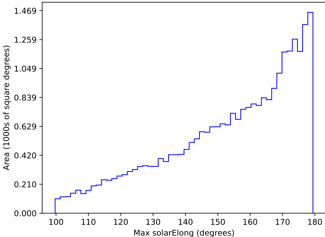
noroll_mjdp60_v3.4_10yrs All sky r band: Max solarElong
