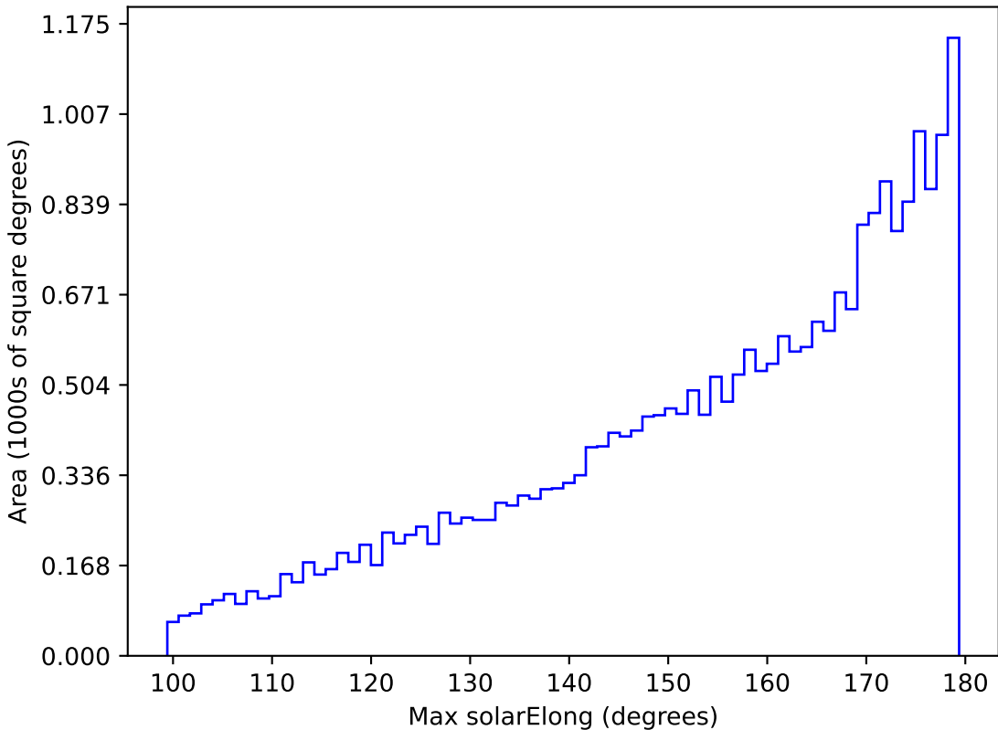
noroll_mjdp60_v3.4_10yrs All sky i band: Max solarElong
