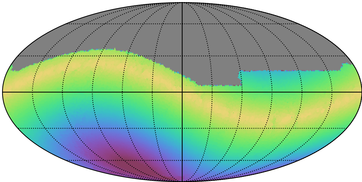
noroll_mjdp60_v3.4_10yrs All sky g band: Max solarElong
