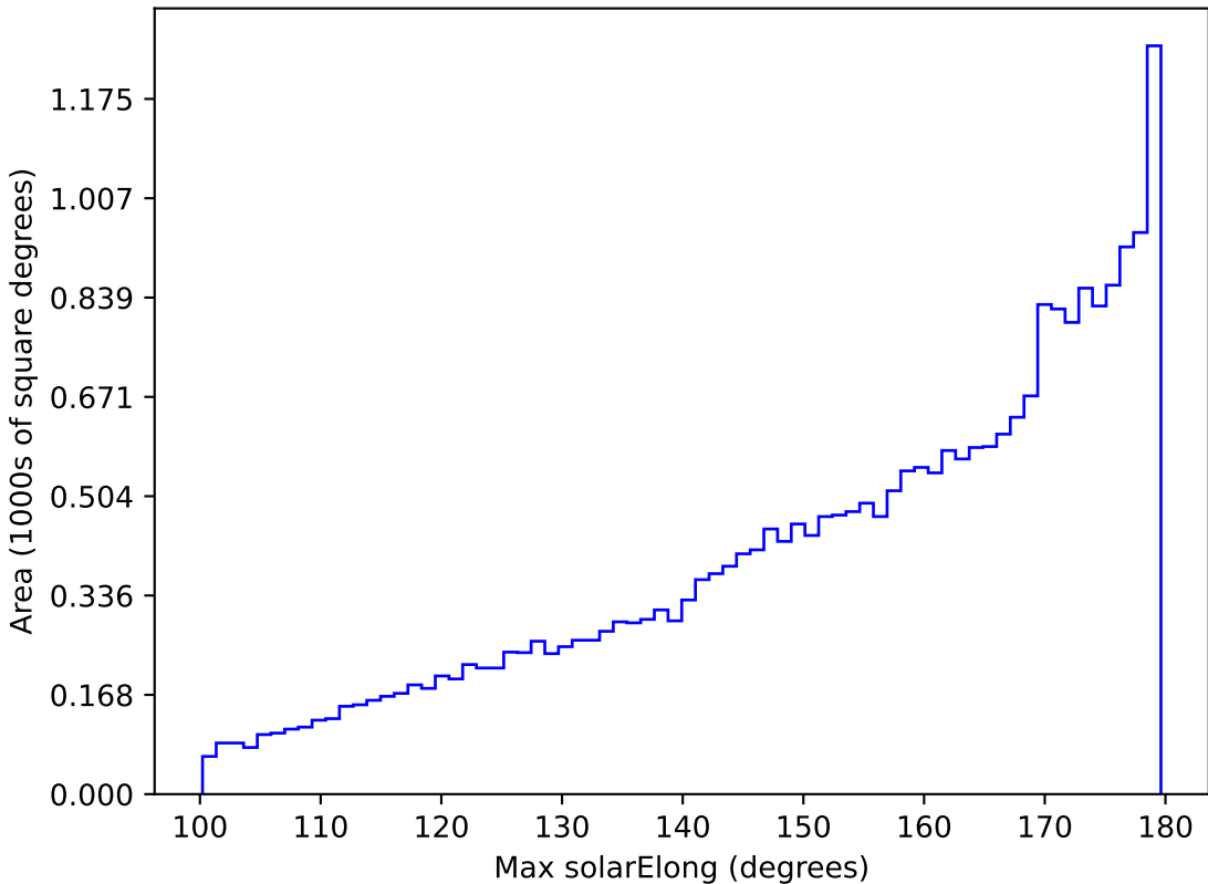
noroll_mjdp60_v3.4_10yrs All sky all bands: Max solarElong
