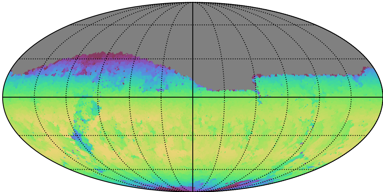
noroll_mjdp60_v3.4_10yrs Yr 1 z band: Max skyBrightness
