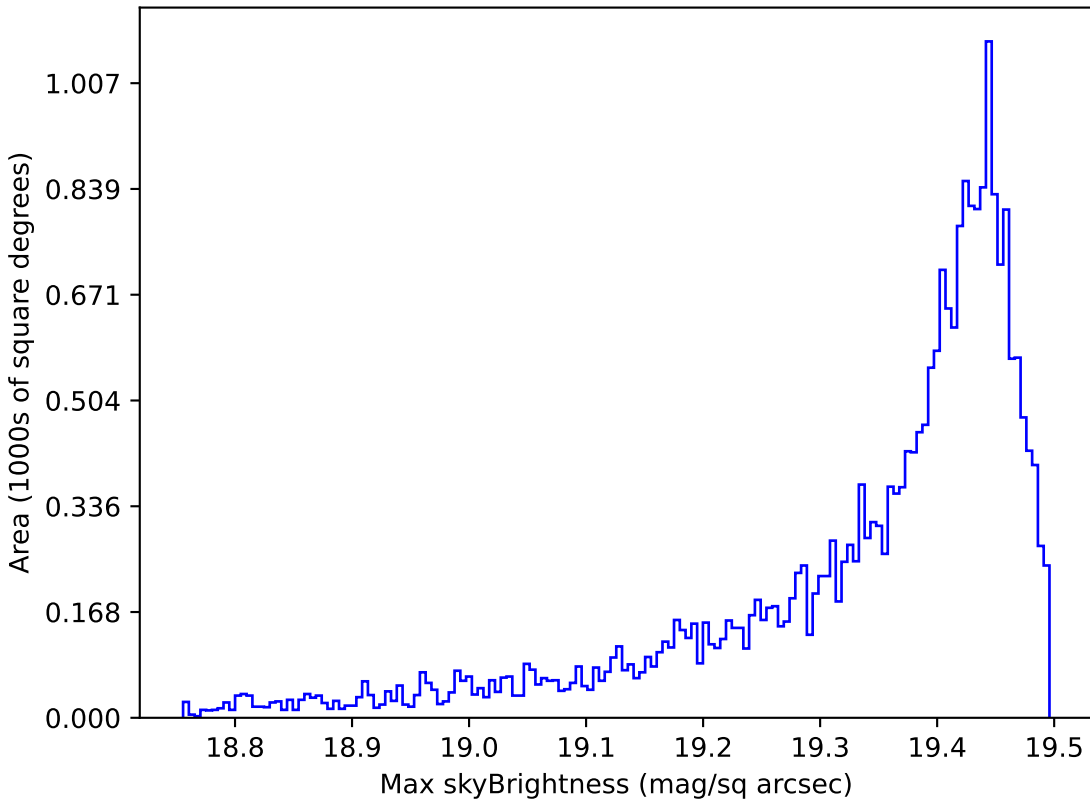
noroll_mjdp60_v3.4_10yrs Yr 1 z band: Max skyBrightness
