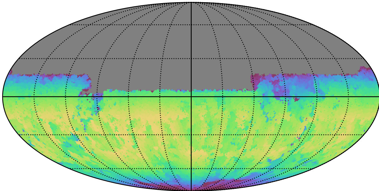
noroll_mjdp60_v3.4_10yrs Yr 1 y band: Max skyBrightness
