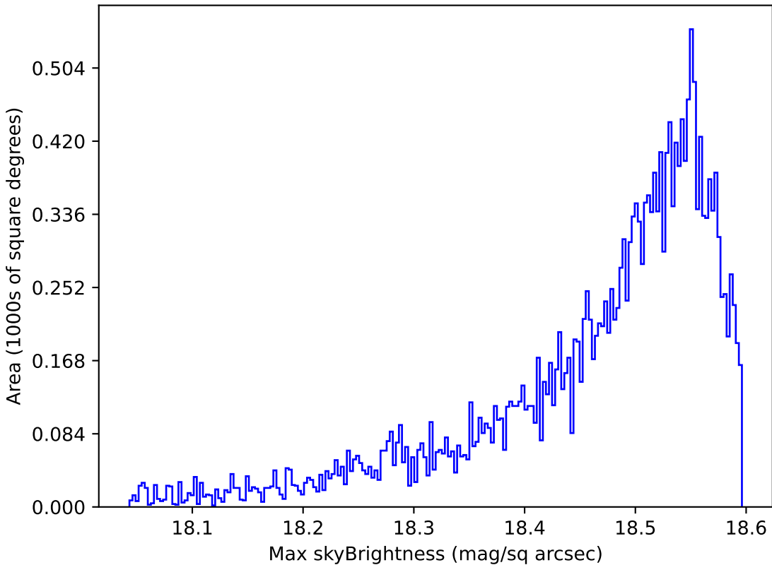
noroll_mjdp60_v3.4_10yrs Yr 1 y band: Max skyBrightness
