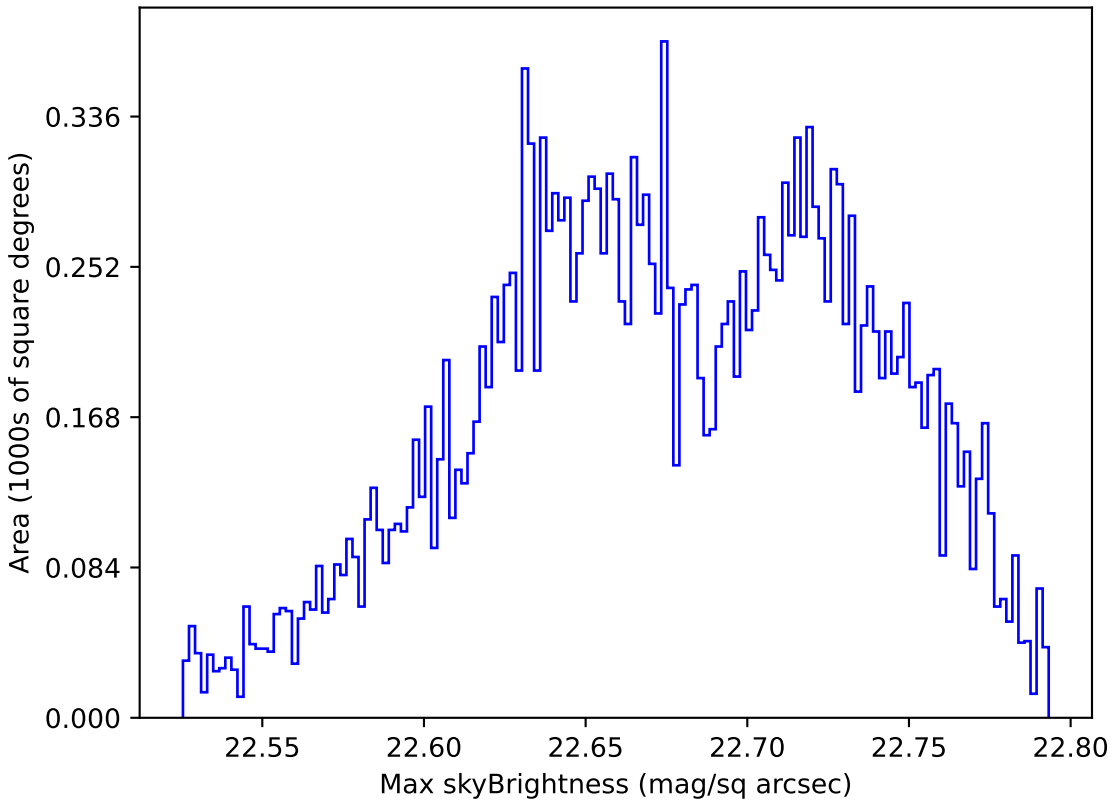
noroll_mjdp60_v3.4_10yrs Yr 1 u band: Max skyBrightness
