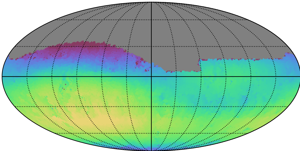
noroll_mjdp60_v3.4_10yrs Yr 1 r band: Max skyBrightness
