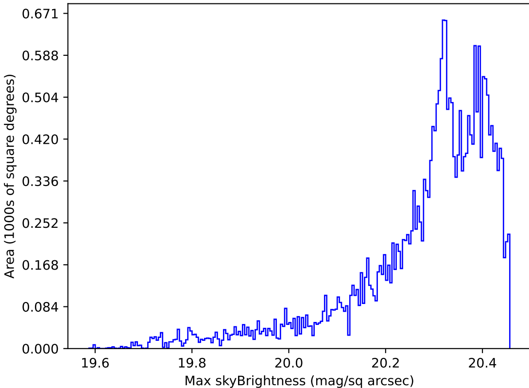
noroll_mjdp60_v3.4_10yrs Yr 1 i band: Max skyBrightness
