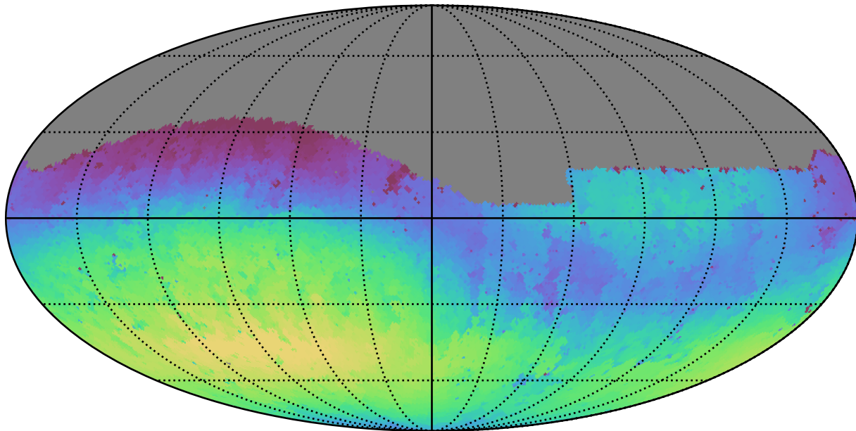
noroll_mjdp60_v3.4_10yrs Yr 1 g band: Max skyBrightness
