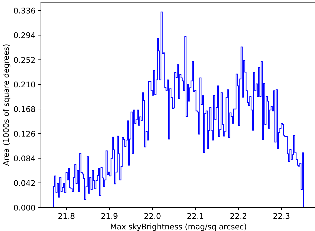
noroll_mjdp60_v3.4_10yrs Yr 1 g band: Max skyBrightness
