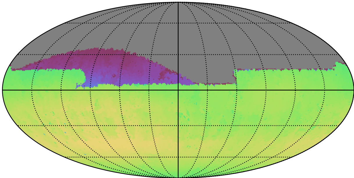
noroll_mjdp60_v3.4_10yrs Yr 1 all bands: Max skyBrightness
