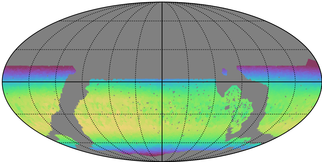
noroll_mjdp60_v3.4_10yrs WFD z band: Max skyBrightness
