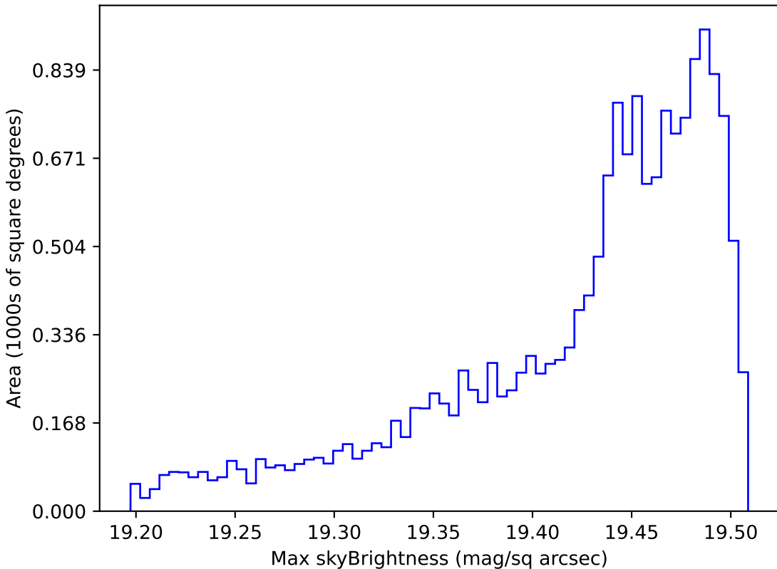
noroll_mjdp60_v3.4_10yrs WFD z band: Max skyBrightness
