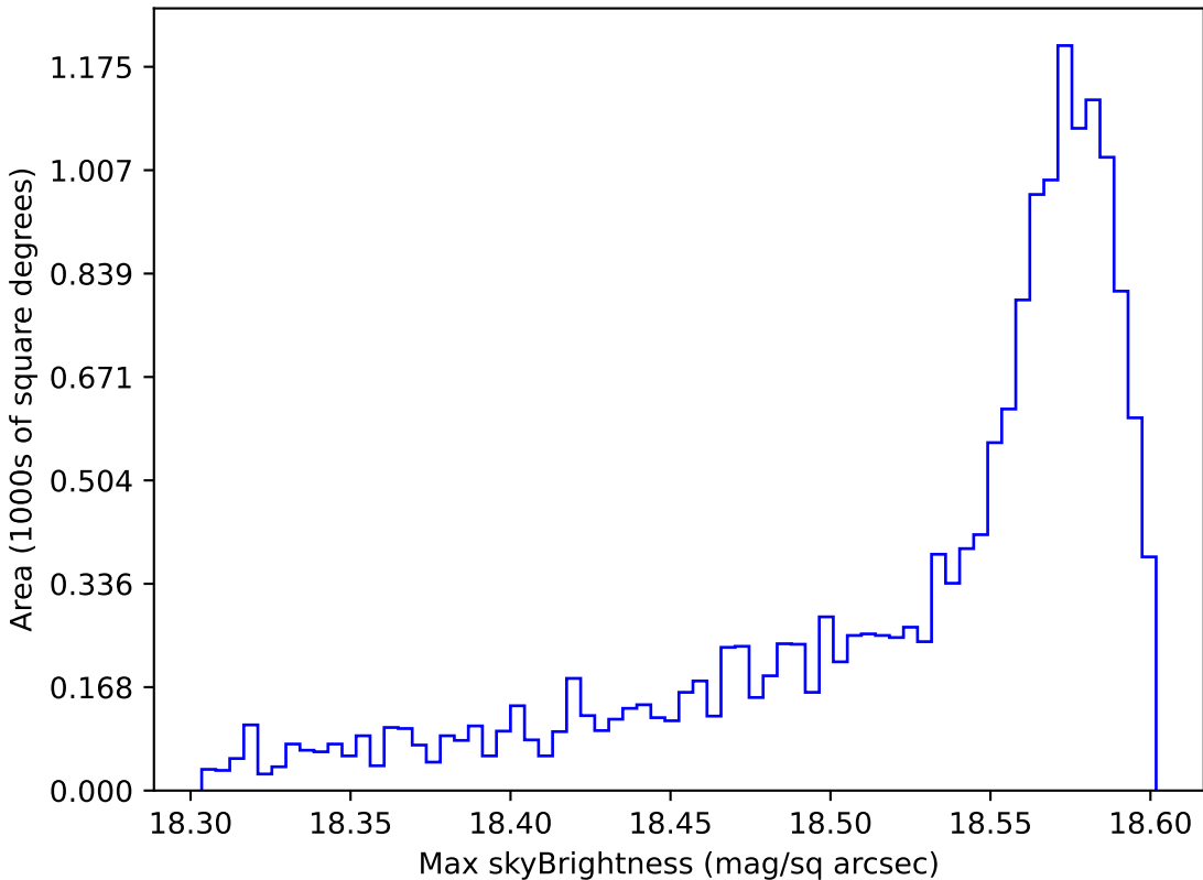
noroll_mjdp60_v3.4_10yrs WFD y band: Max skyBrightness
