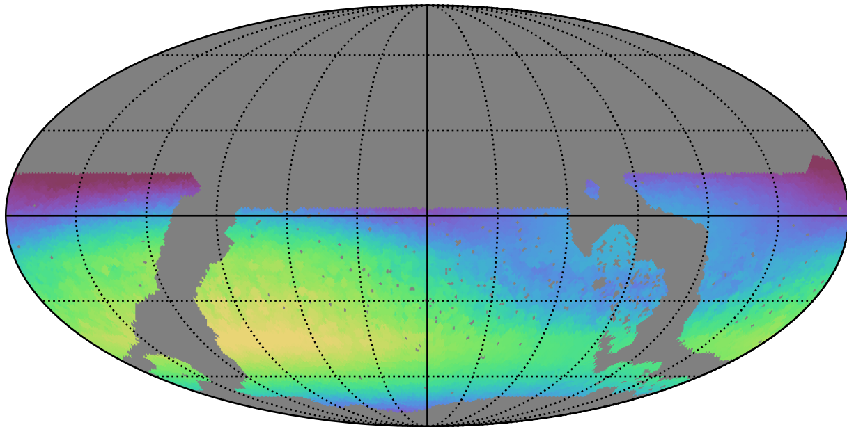
noroll_mjdp60_v3.4_10yrs WFD u band: Max skyBrightness
