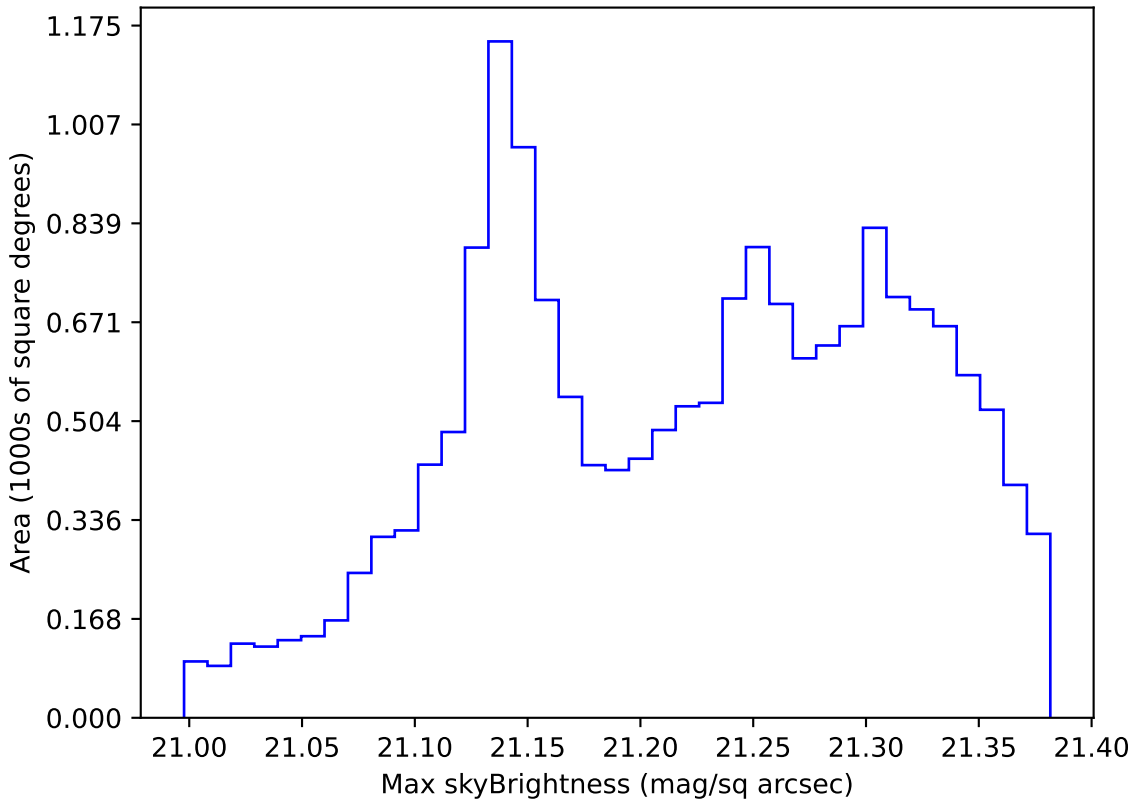
noroll_mjdp60_v3.4_10yrs WFD r band: Max skyBrightness
