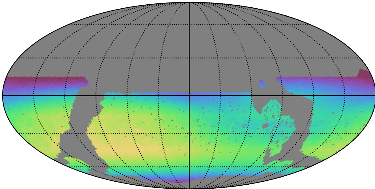
noroll_mjdp60_v3.4_10yrs WFD i band: Max skyBrightness
