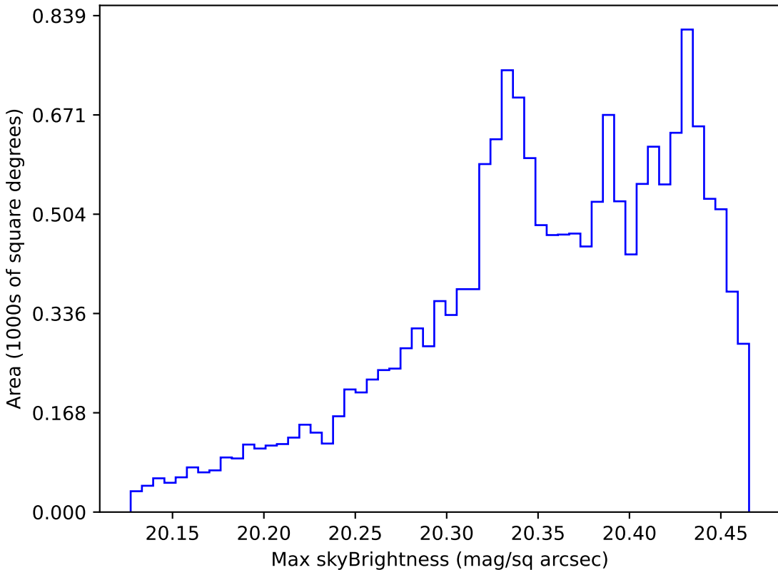
noroll_mjdp60_v3.4_10yrs WFD i band: Max skyBrightness
