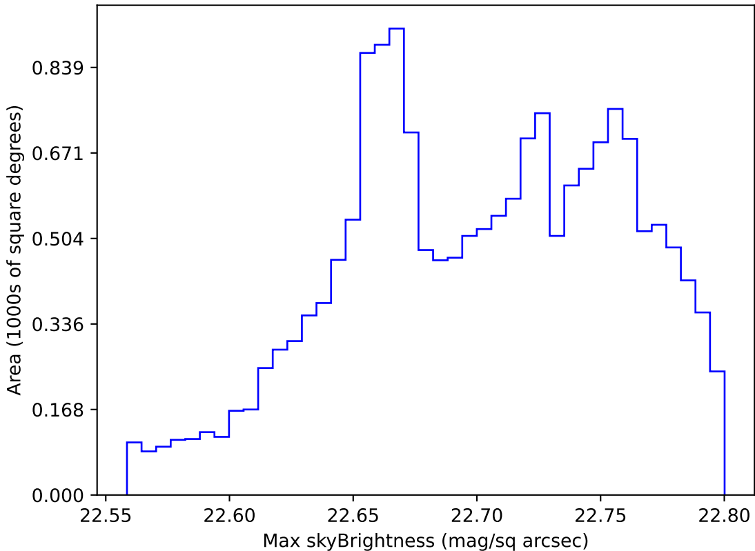
noroll_mjdp60_v3.4_10yrs WFD all bands: Max skyBrightness
