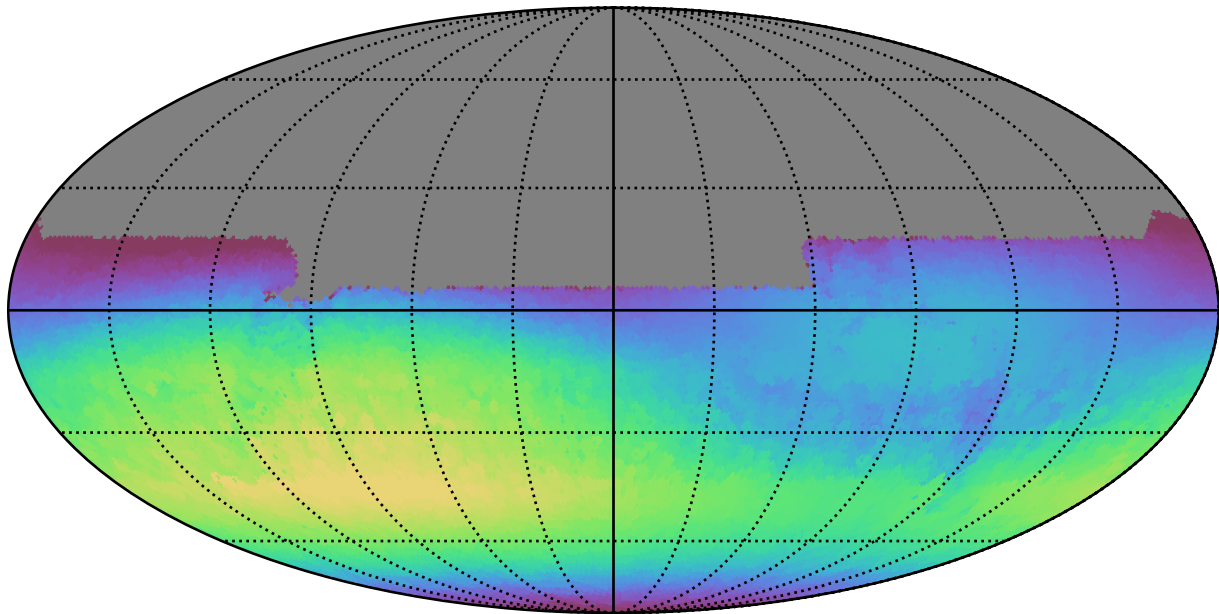
noroll_mjdp60_v3.4_10yrs All sky u band: Max skyBrightness
