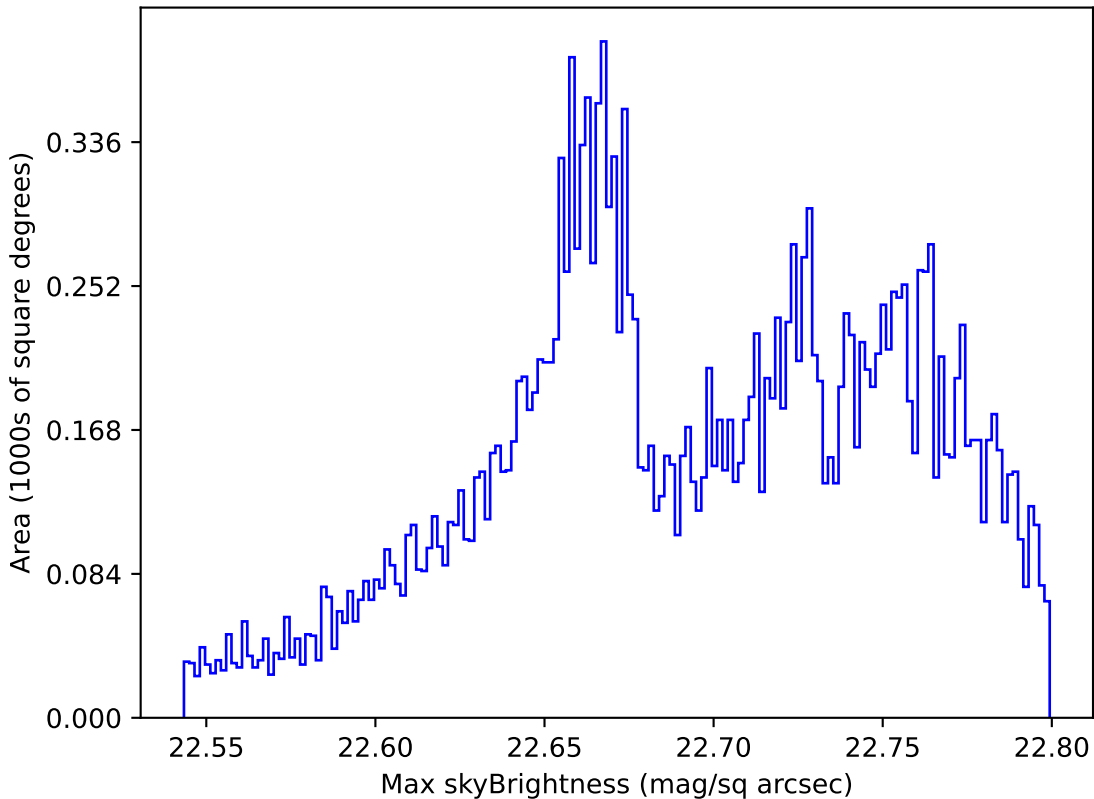
noroll_mjdp60_v3.4_10yrs All sky u band: Max skyBrightness
