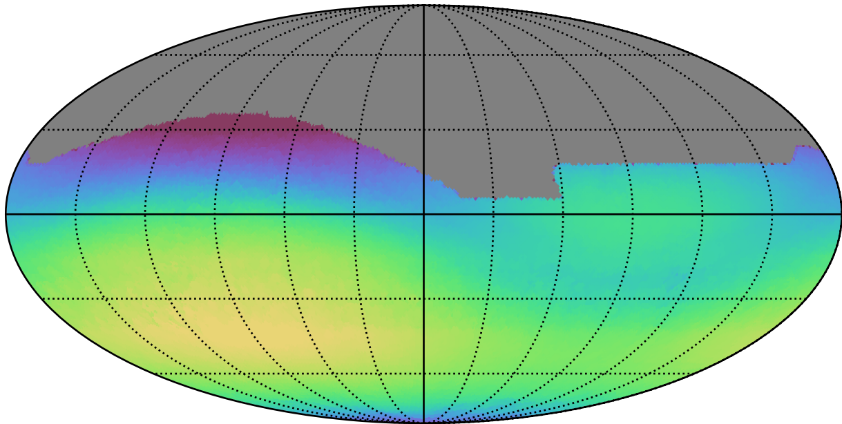
noroll_mjdp60_v3.4_10yrs All sky r band: Max skyBrightness
