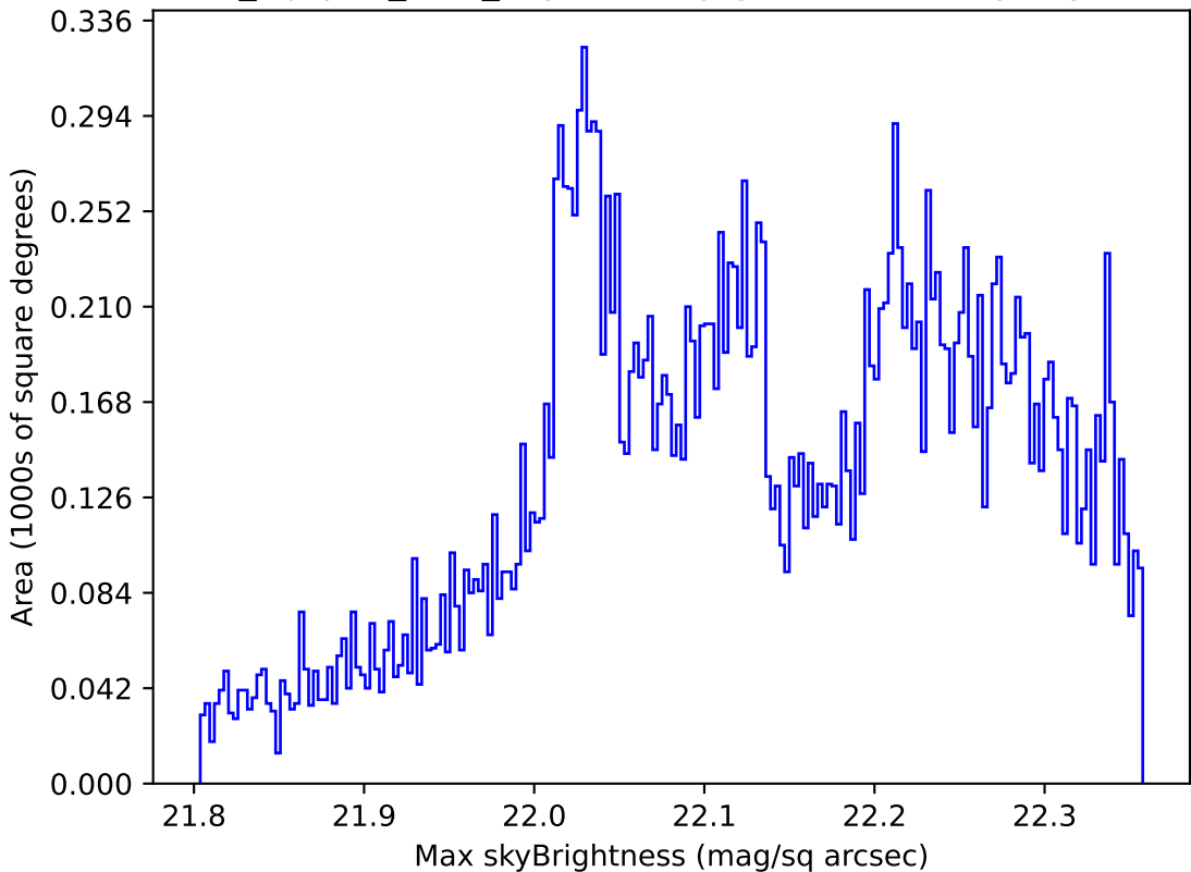
noroll_mjdp60_v3.4_10yrs All sky g band: Max skyBrightness
