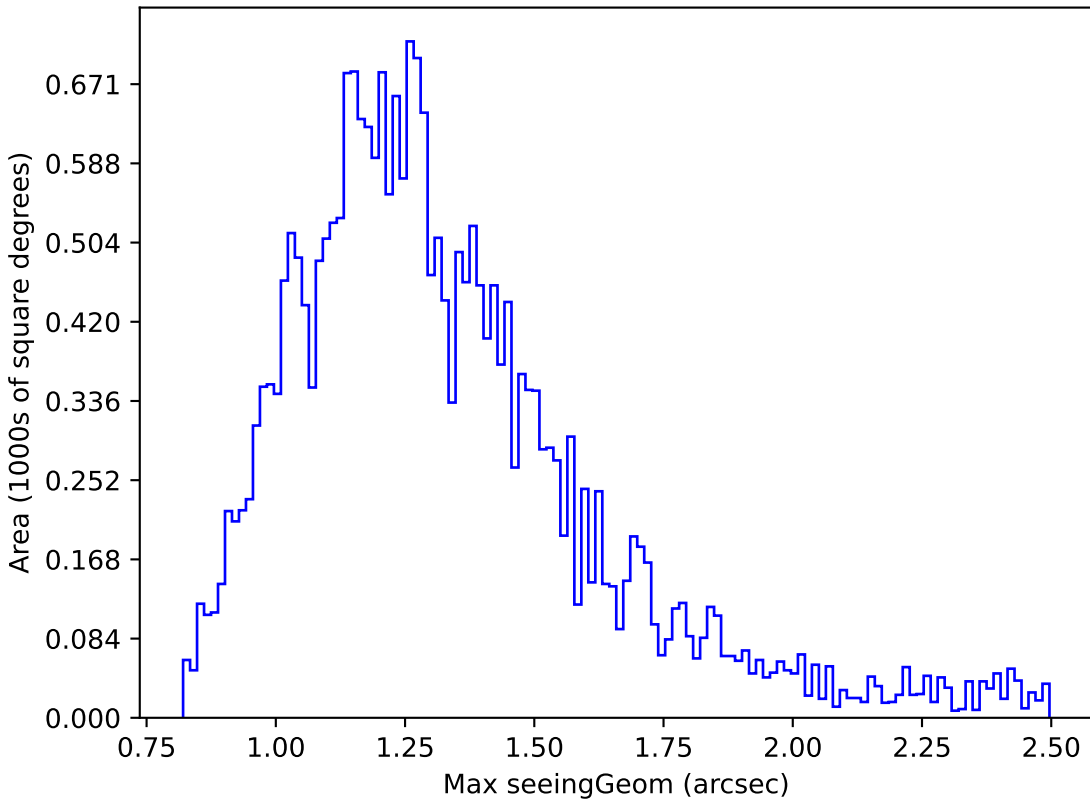
noroll_mjdp60_v3.4_10yrs Yr 1 z band: Max seeingGeom
