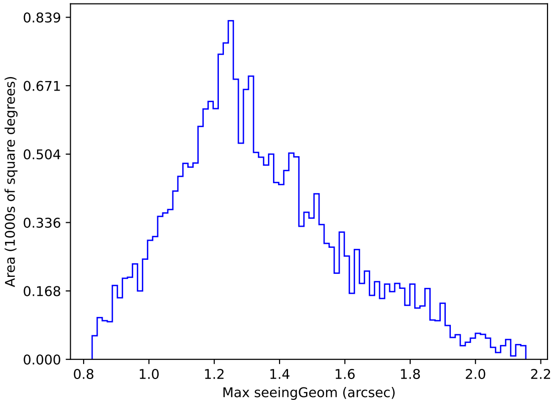
noroll_mjdp60_v3.4_10yrs Yr 1 u band: Max seeingGeom
