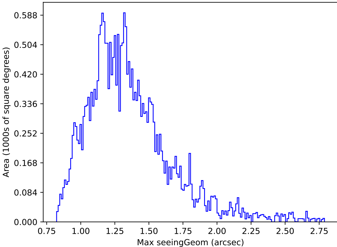
noroll_mjdp60_v3.4_10yrs Yr 1 i band: Max seeingGeom
