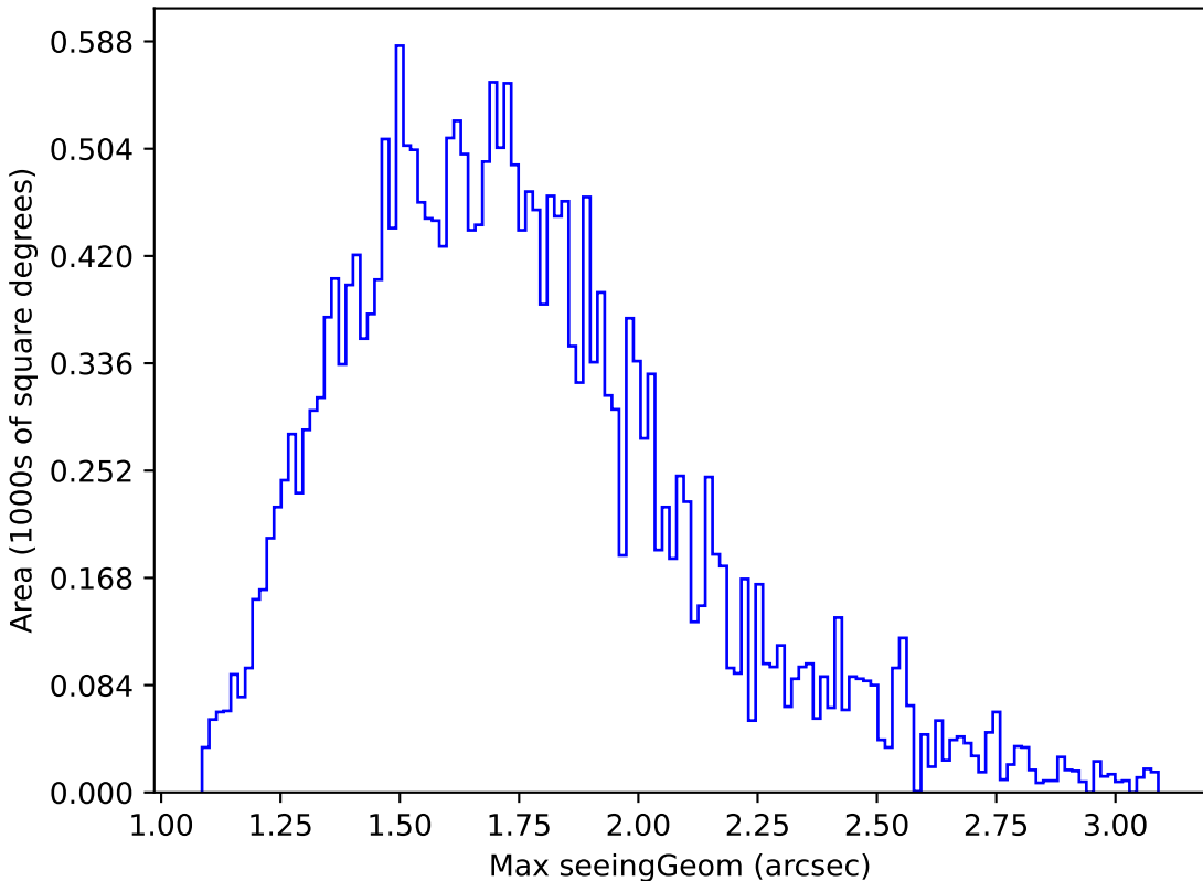
noroll_mjdp60_v3.4_10yrs Yr 1 all bands: Max seeingGeom
