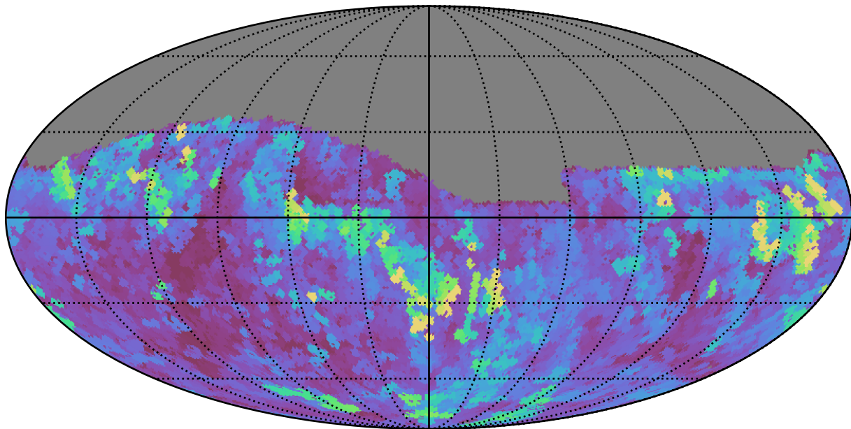
noroll_mjdp60_v3.4_10yrs Yr 1 z band: Max seeingEff
