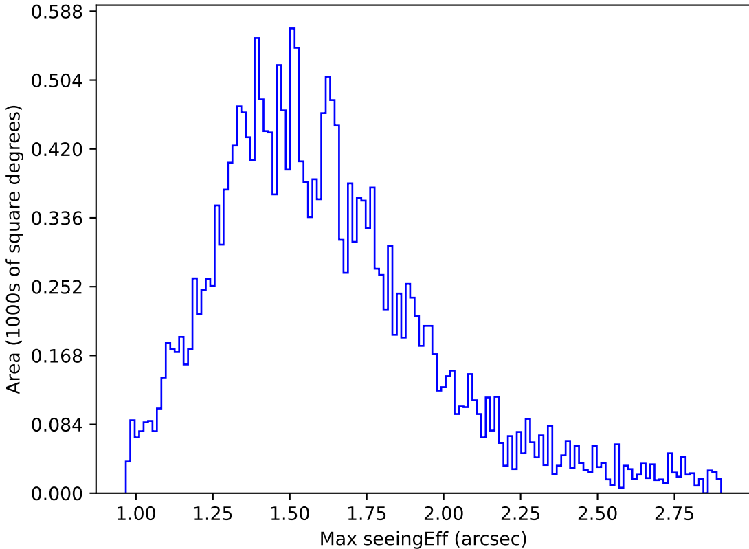
noroll_mjdp60_v3.4_10yrs Yr 1 y band: Max seeingEff
