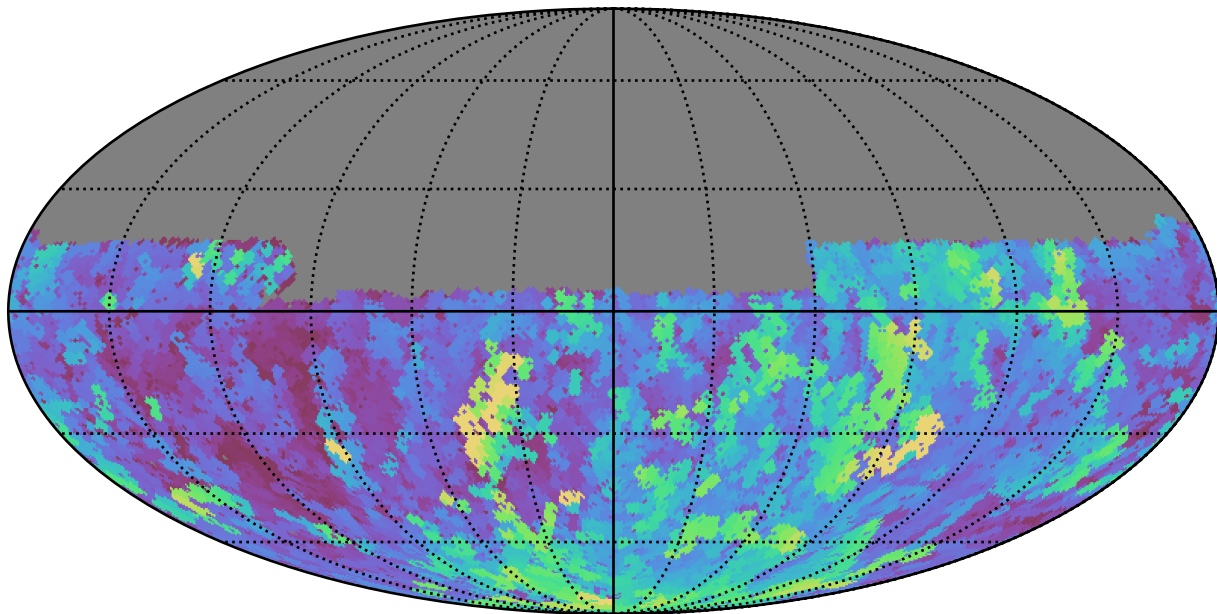
noroll_mjdp60_v3.4_10yrs Yr 1 u band: Max seeingEff
