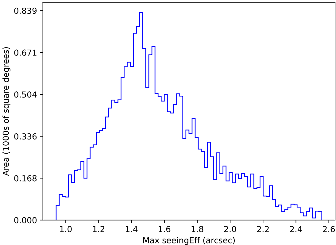
noroll_mjdp60_v3.4_10yrs Yr 1 u band: Max seeingEff
