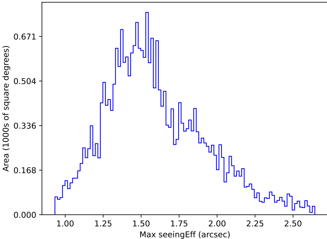
noroll_mjdp60_v3.4_10yrs Yr 1 r band: Max seeingEff
