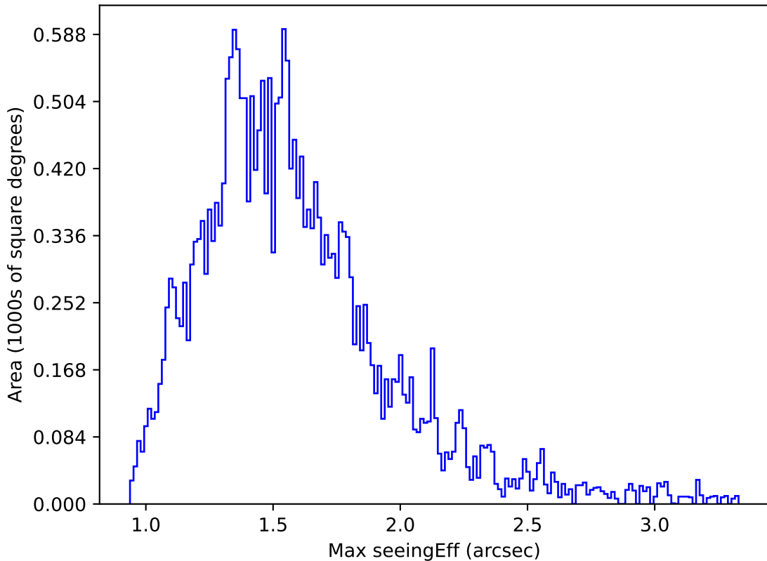
noroll_mjdp60_v3.4_10yrs Yr 1 i band: Max seeingEff
