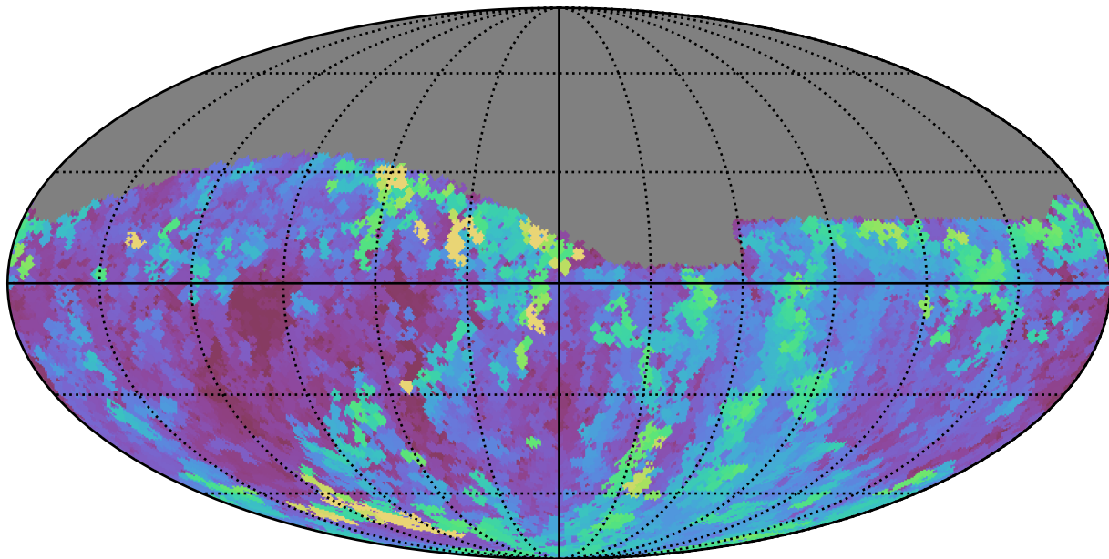
noroll_mjdp60_v3.4_10yrs Yr 1 g band: Max seeingEff
