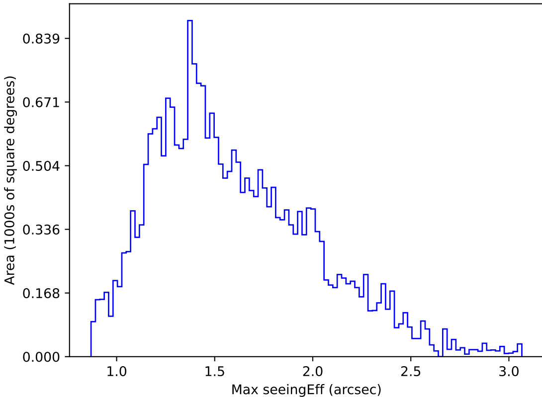
noroll_mjdp60_v3.4_10yrs Yr 1 g band: Max seeingEff
