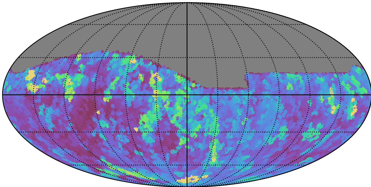
noroll_mjdp60_v3.4_10yrs Yr 1 all bands: Max seeingEff
