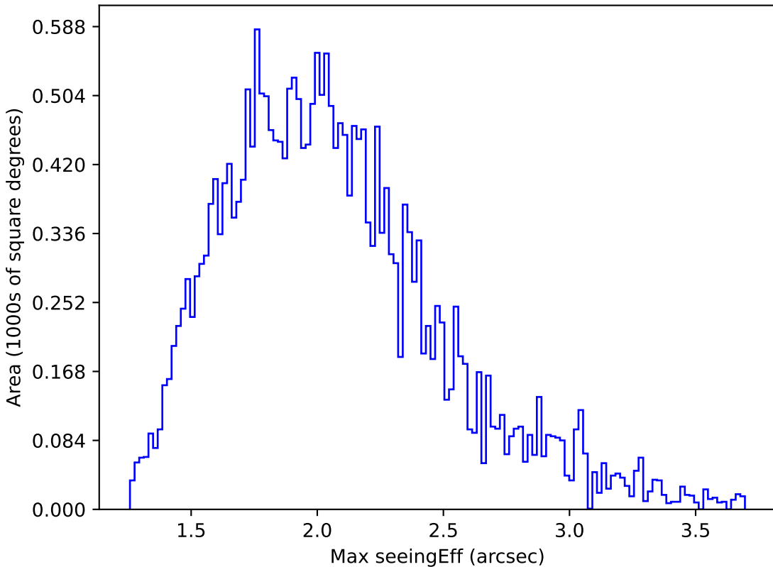
noroll_mjdp60_v3.4_10yrs Yr 1 all bands: Max seeingEff
