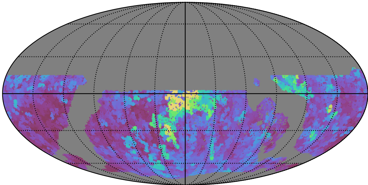
noroll_mjdp60_v3.4_10yrs WFD y band: Max seeingEff
