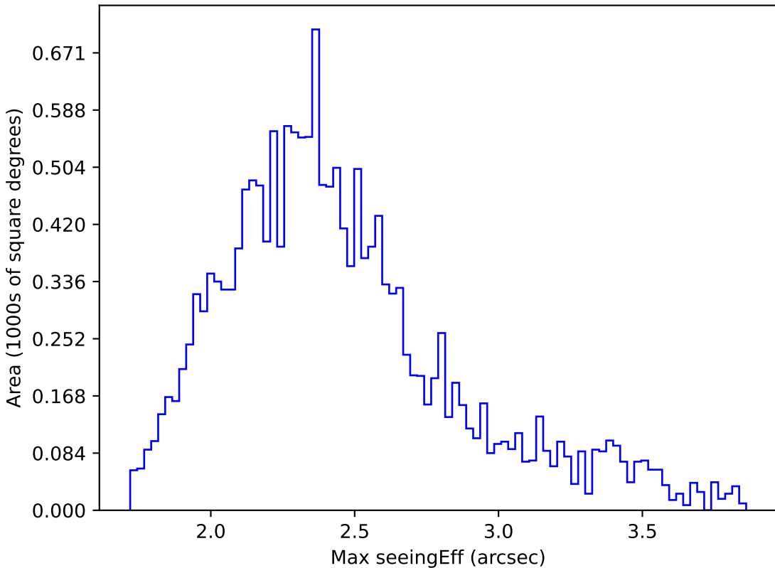
noroll_mjdp60_v3.4_10yrs WFD u band: Max seeingEff
