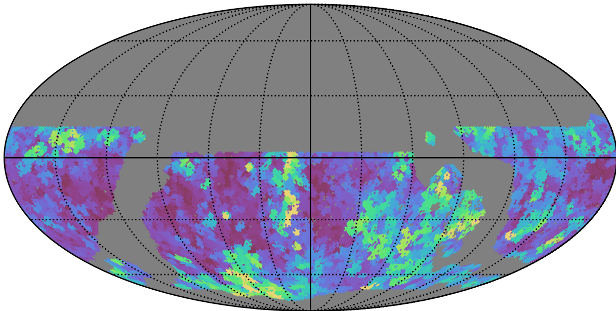
noroll_mjdp60_v3.4_10yrs WFD g band: Max seeingEff
