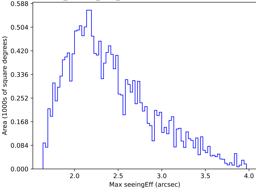
noroll_mjdp60_v3.4_10yrs WFD g band: Max seeingEff
