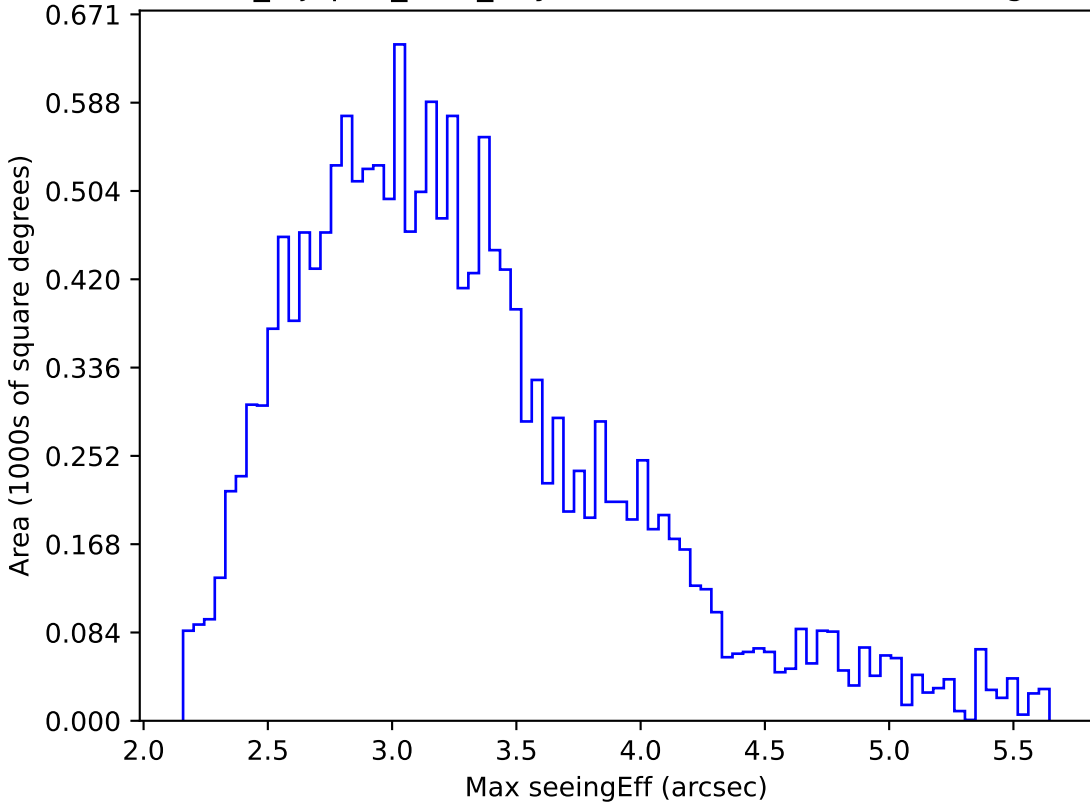
noroll_mjdp60_v3.4_10yrs WFD all bands: Max seeingEff
