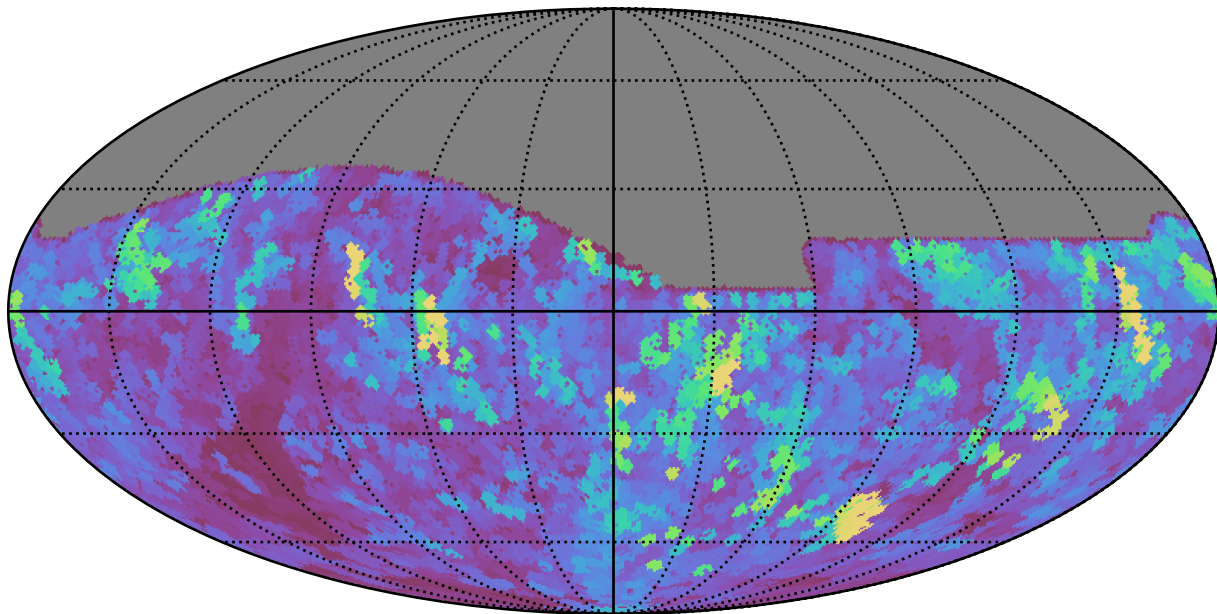
noroll_mjdp60_v3.4_10yrs All sky z band: Max seeingEff
