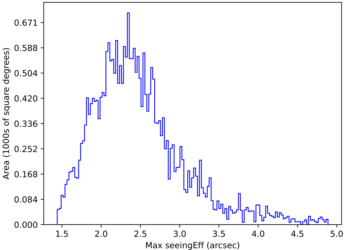
noroll_mjdp60_v3.4_10yrs All sky z band: Max seeingEff
