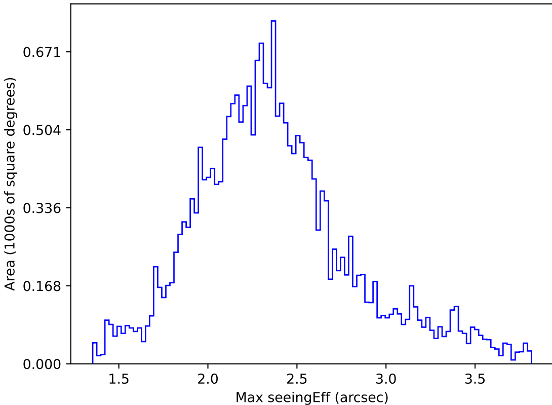
noroll_mjdp60_v3.4_10yrs All sky u band: Max seeingEff
